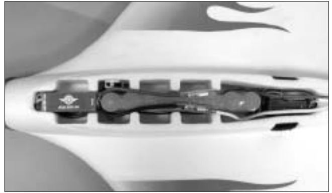
23. Connect all wires to receiver then place ESC, Battery and Receiver as shown.
